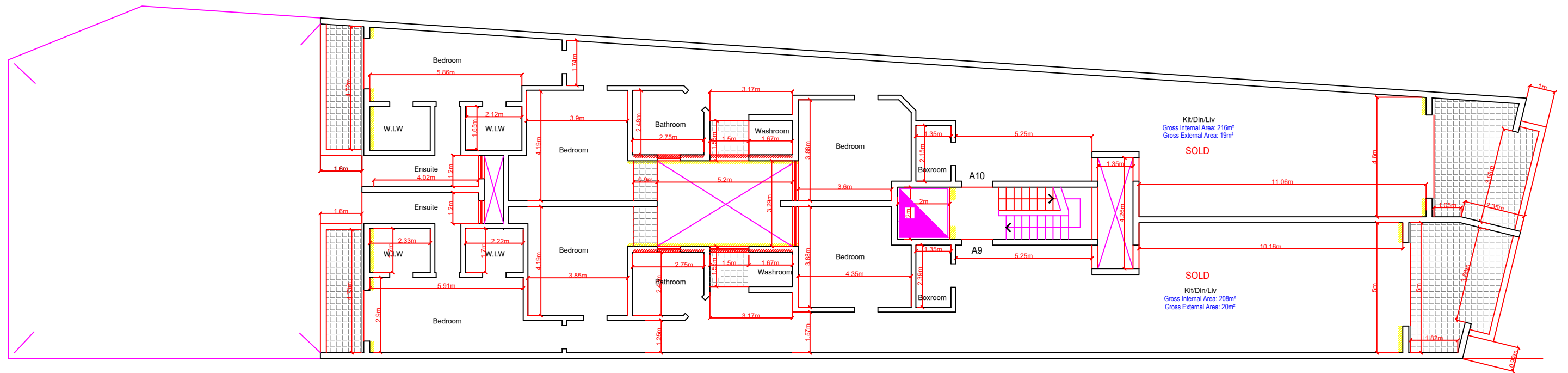
Proposed Fifth Floor
